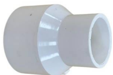
PVC PRESS REDUC SOCKET 100mm X 50mm
